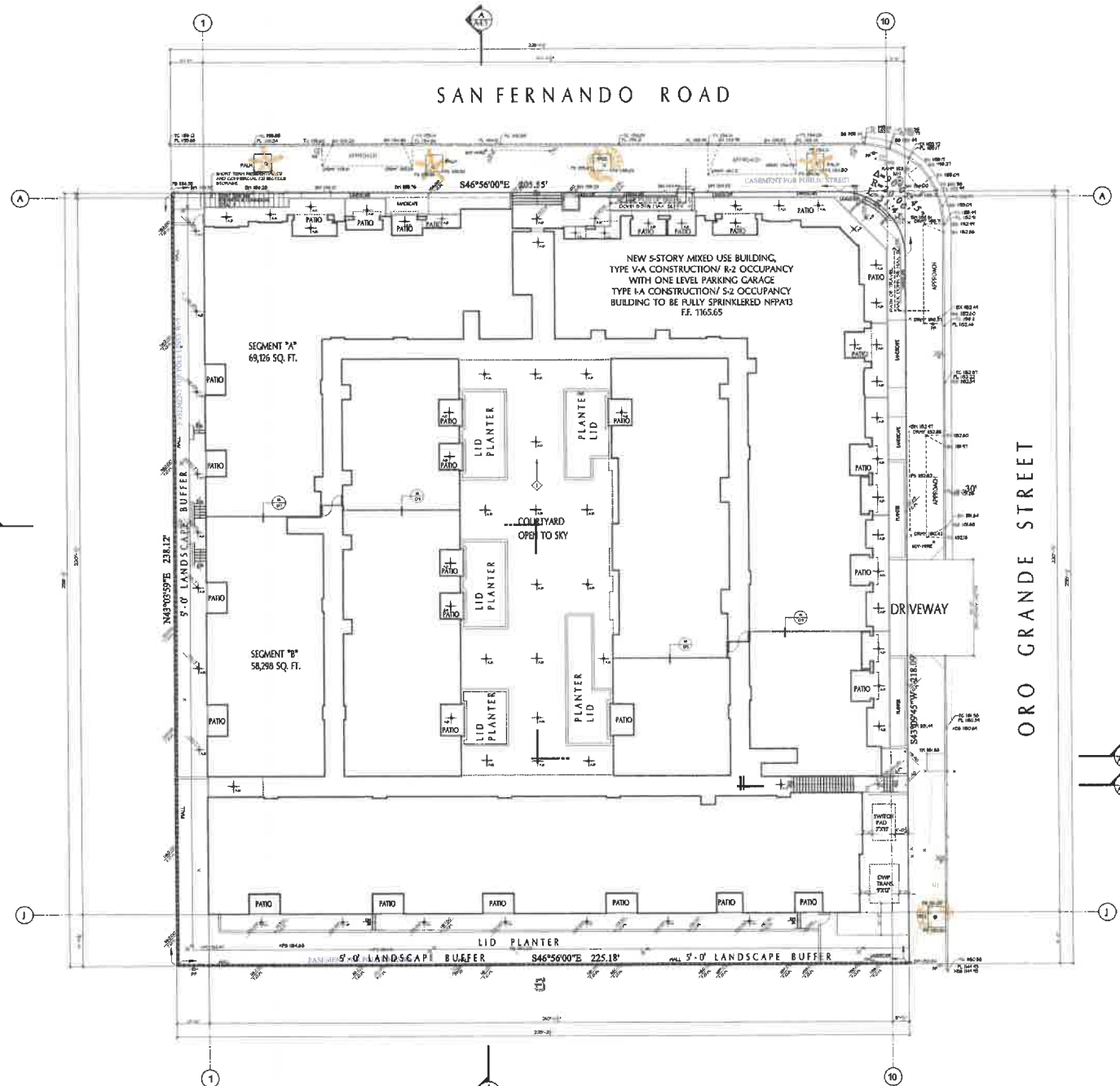
SITE PLAN ACCESSIBLE BUILDING
